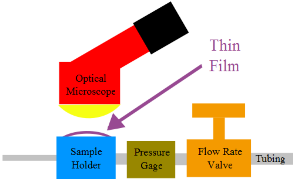
Figure 3-1 Bulge testing experimental setup. An optical microscope was used to measure the deflection of the thin film in the normal direction. A pressure gauge was used to measure the pressure and the pressure was controlled using a flow rate valve.
