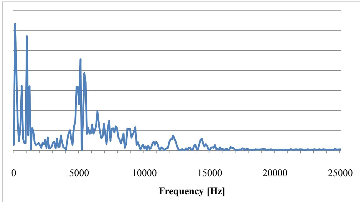
Figure 5-3 Fourier transform spectrum of mechanical shock wave. The dominate frequencies are in the 10^3 to 10^4 range.
